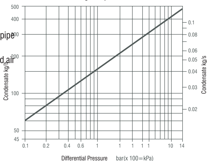
Discharge Capacities
